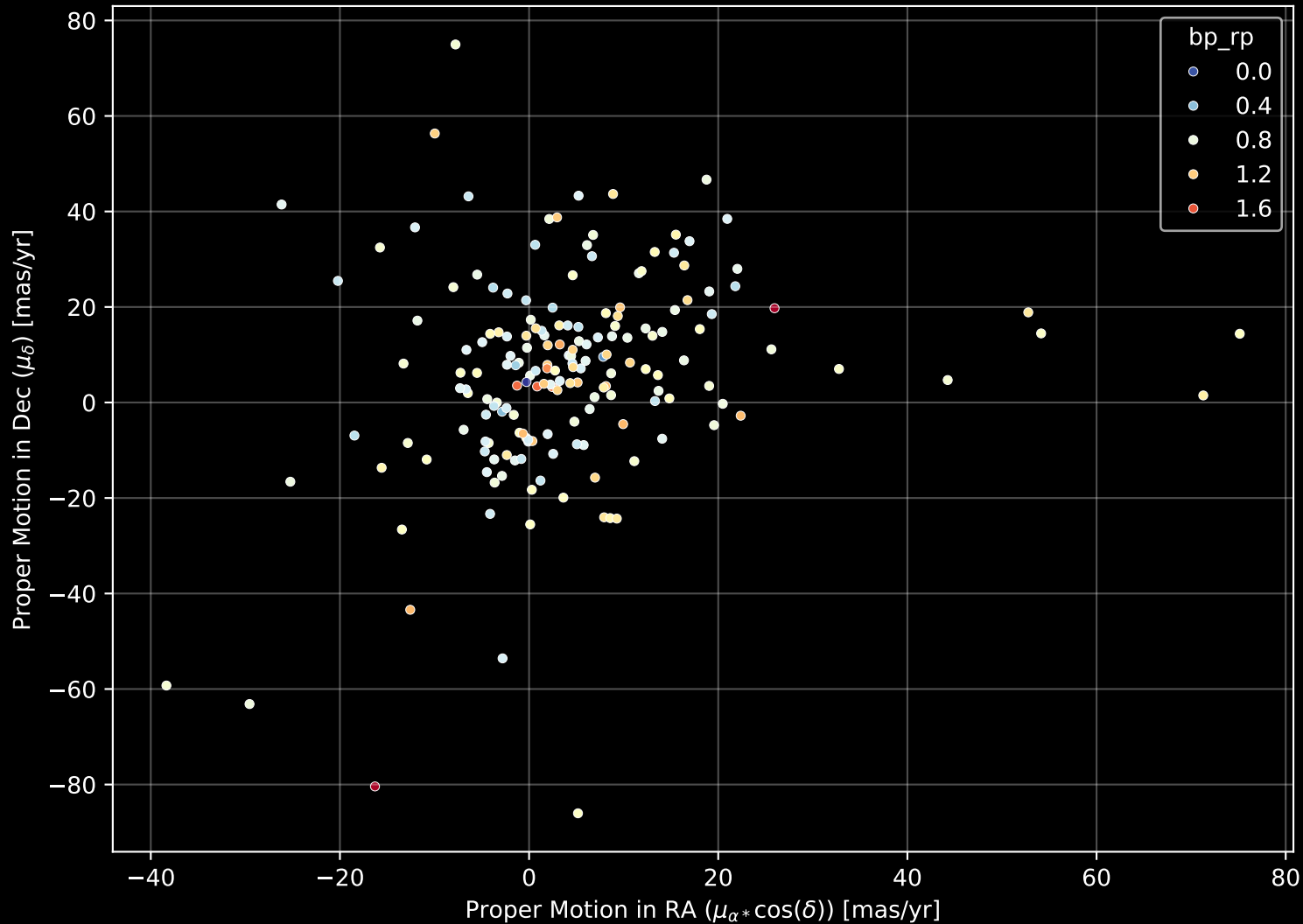
GALAH DR4 Field: [7182] Proper Motion Diagram (n= 179)
