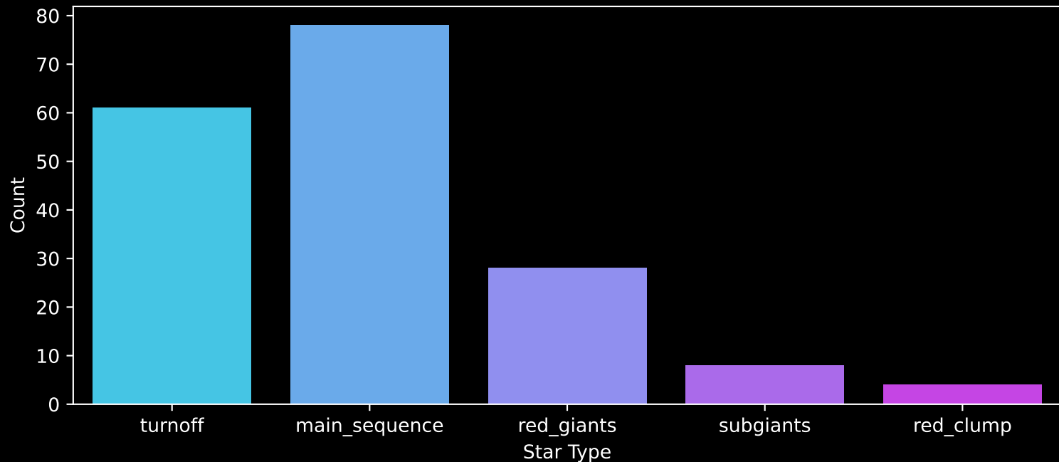
GALAH DR4 Field: [7182] Count plot of Star Type
