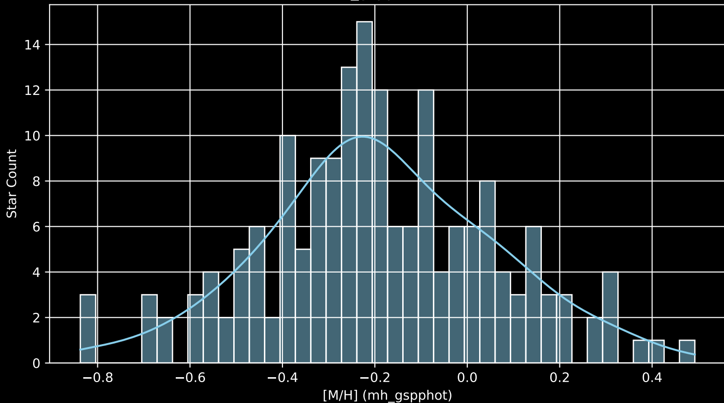
GALAH DR4 Field: [7182] [M/H] (mh_gspphot) (n= 179)
