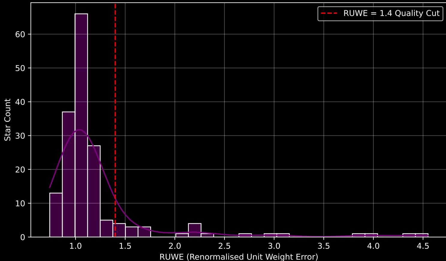
GALAH DR4 Field [7182] RUWE Distribution (n= 171)
