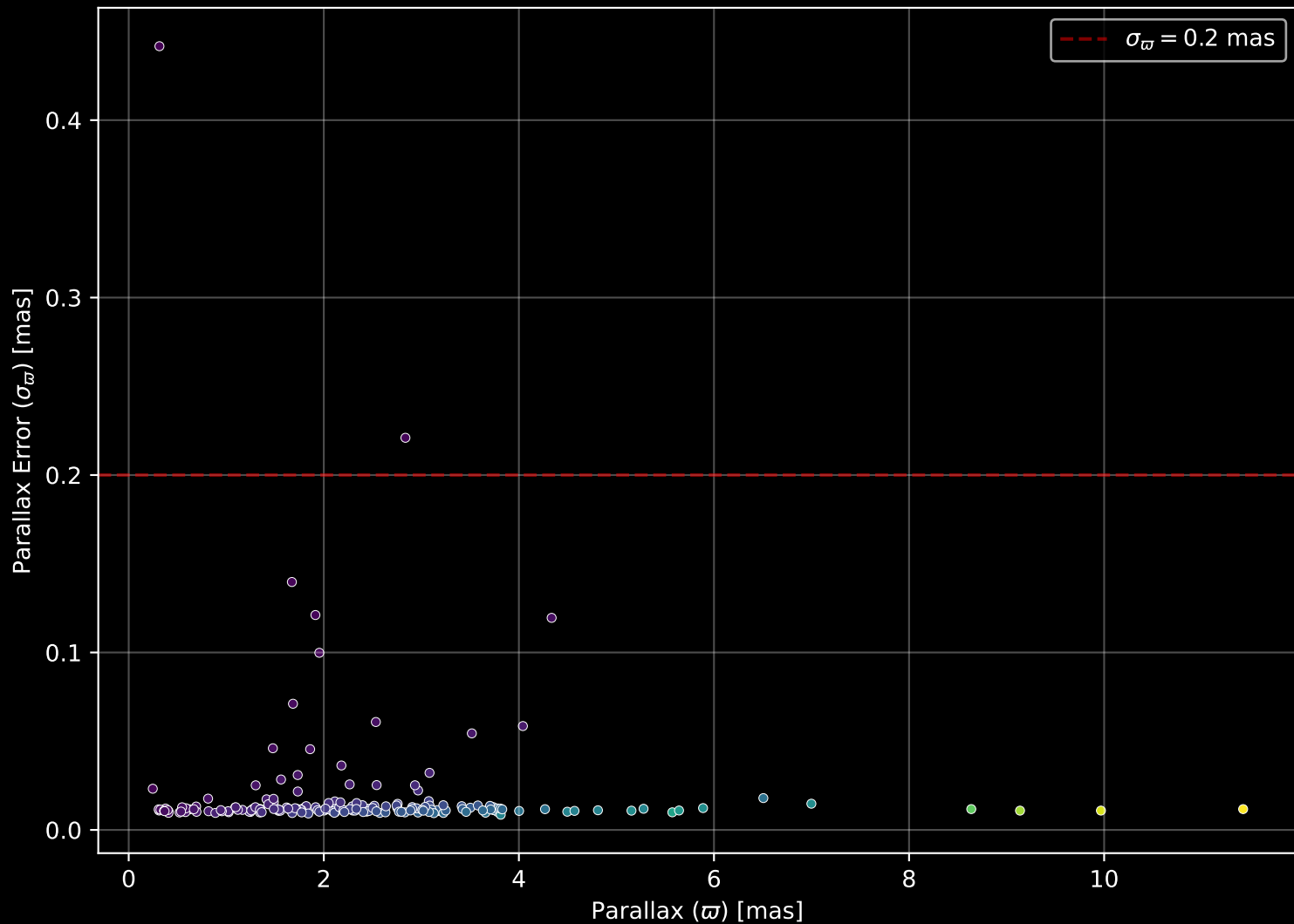
GALAH DR4 Field: [7182] Parallax Quality (n= 179)
