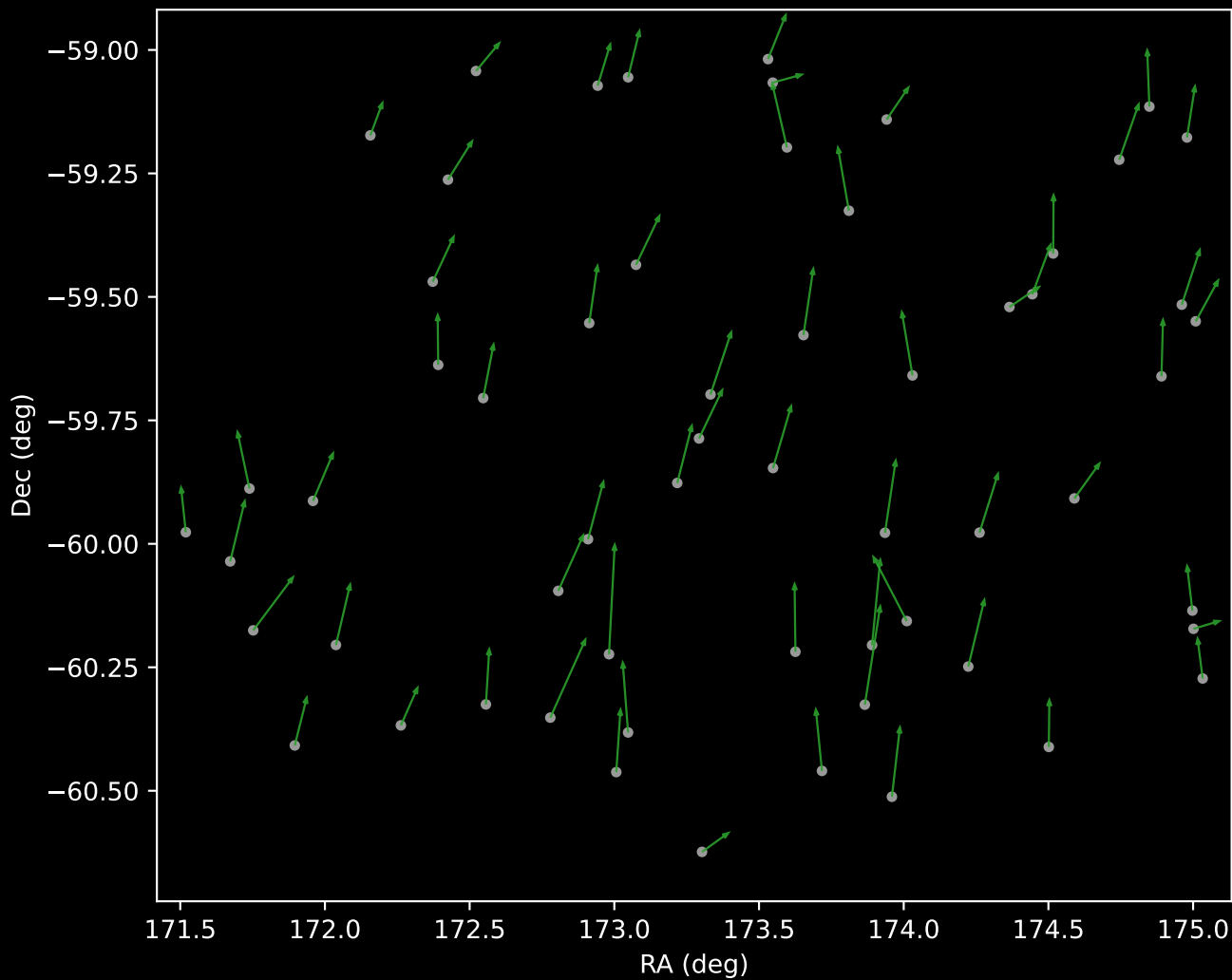
GALAH DR4 Cluster 4 Proper Motion Vectors (n=60)
